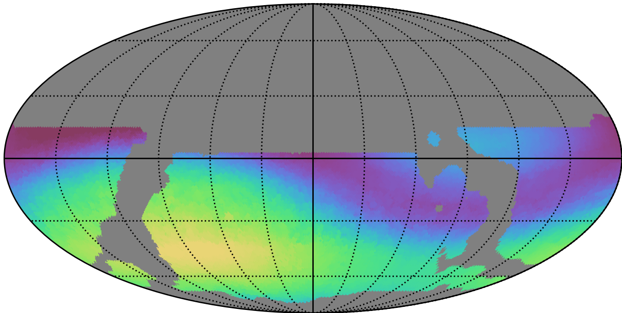
weather_cloudso20v3.4_10yrs WFD g band: Max skyBrightness
