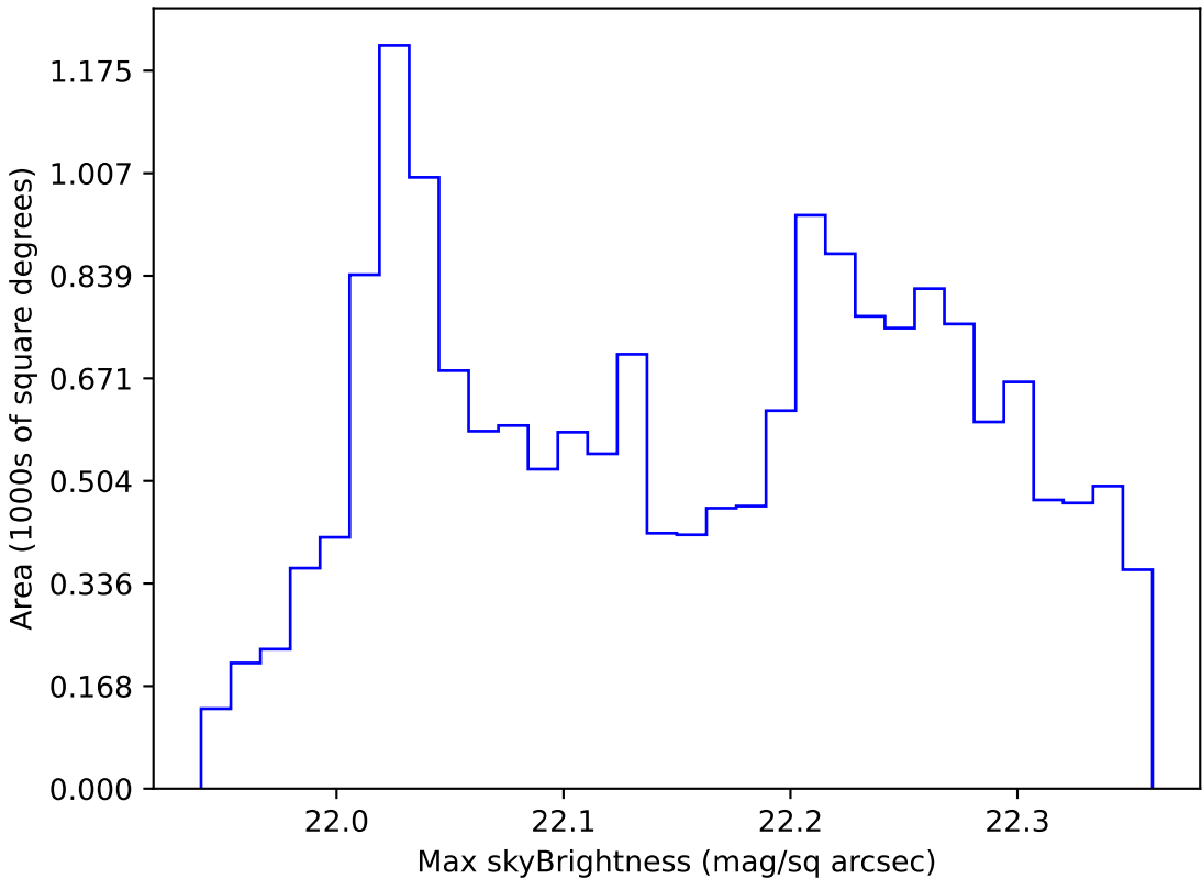
weather_cloudso20v3.4_10yrs WFD g band: Max skyBrightness
