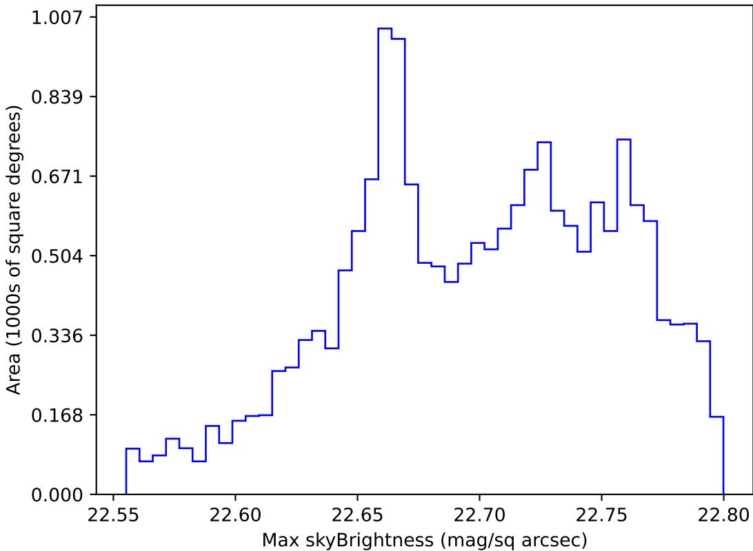
weather_cloudso20v3.4_10yrs WFD all bands: Max skyBrightness
