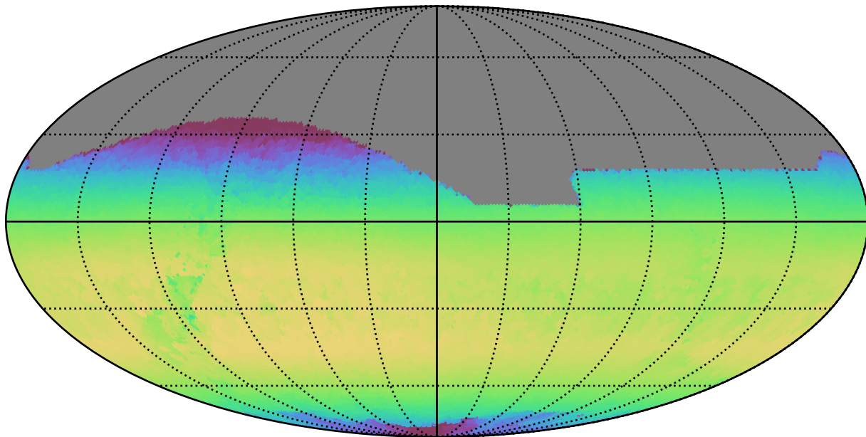
weather_cloudso20v3.4_10yrs All sky z band: Max skyBrightness
