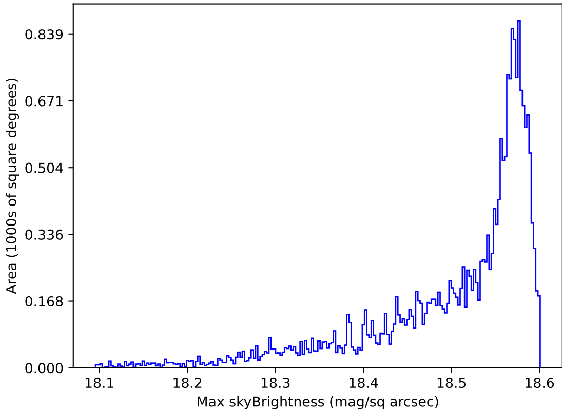
weather_cloudso20v3.4_10yrs All sky y band: Max skyBrightness
