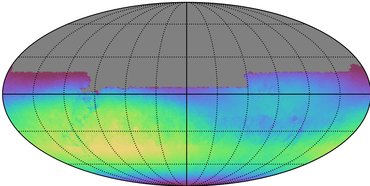
weather_cloudso20v3.4_10yrs All sky u band: Max skyBrightness
