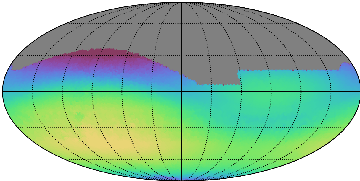
weather_cloudso20v3.4_10yrs All sky r band: Max skyBrightness
