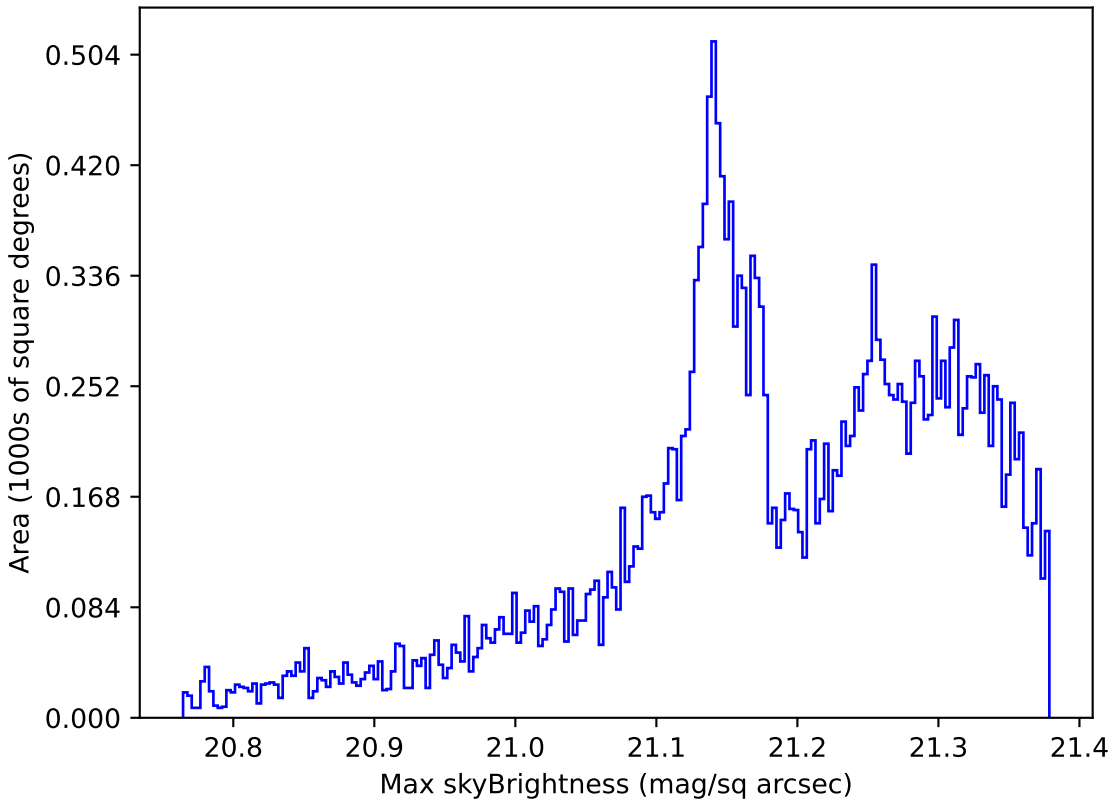
weather_cloudso20v3.4_10yrs All sky r band: Max skyBrightness
