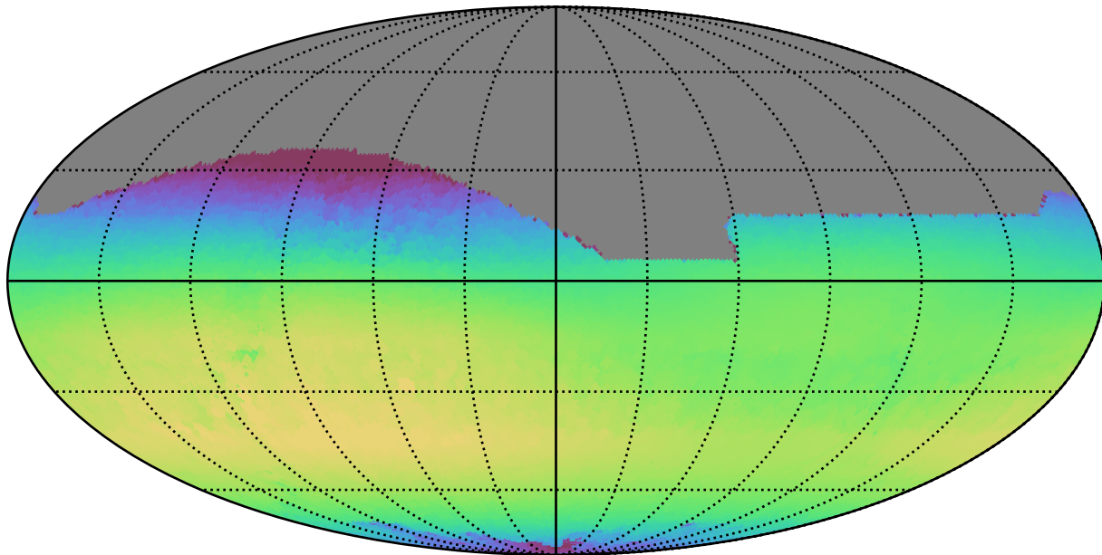
weather_cloudso20v3.4_10yrs All sky i band: Max skyBrightness
