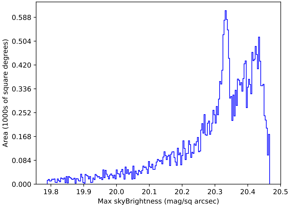
weather_cloudso20v3.4_10yrs All sky i band: Max skyBrightness
