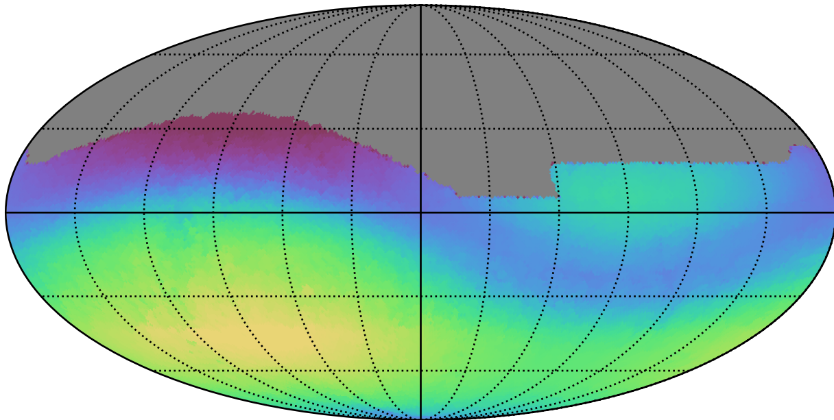
weather_cloudso20v3.4_10yrs All sky g band: Max skyBrightness
