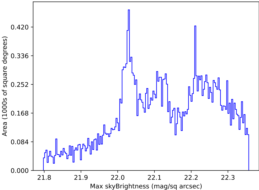
weather_cloudso20v3.4_10yrs All sky g band: Max skyBrightness
