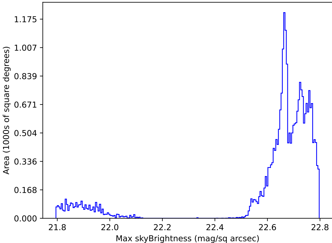
weather_cloudso20v3.4_10yrs All sky all bands: Max skyBrightness
