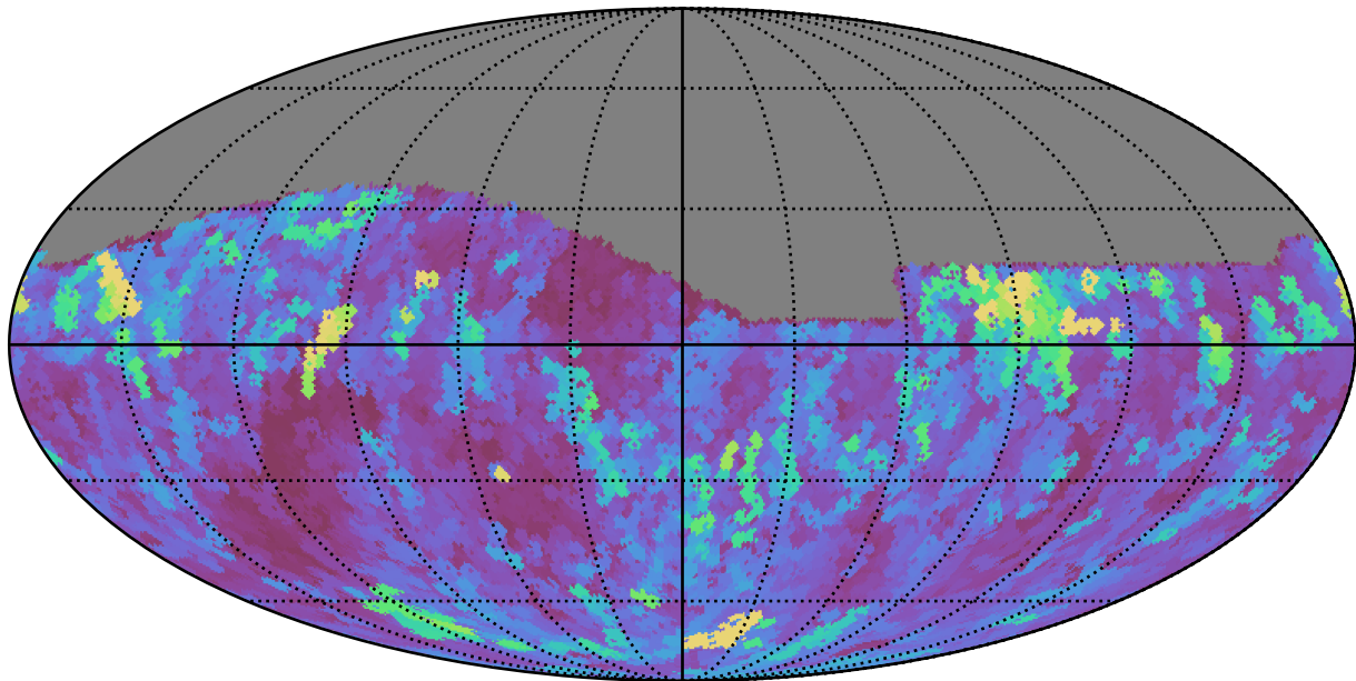
weather_cloudso20v3.4_10yrs Yr 1 all bands: Max seeingGeom
