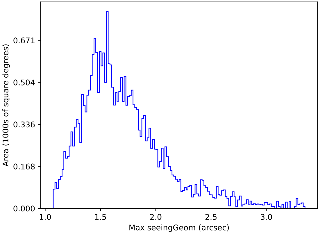
weather_cloudso20v3.4_10yrs Yr 1 all bands: Max seeingGeom
