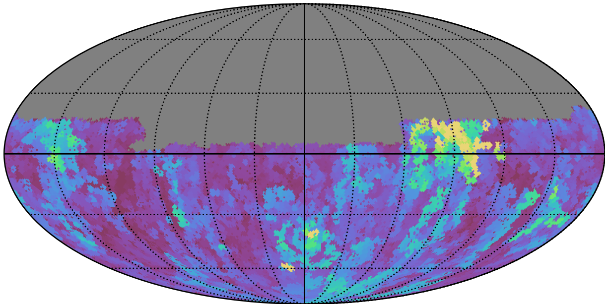
weather_cloudso20v3.4_10yrs Yr 1 u band: Max seeingEff
