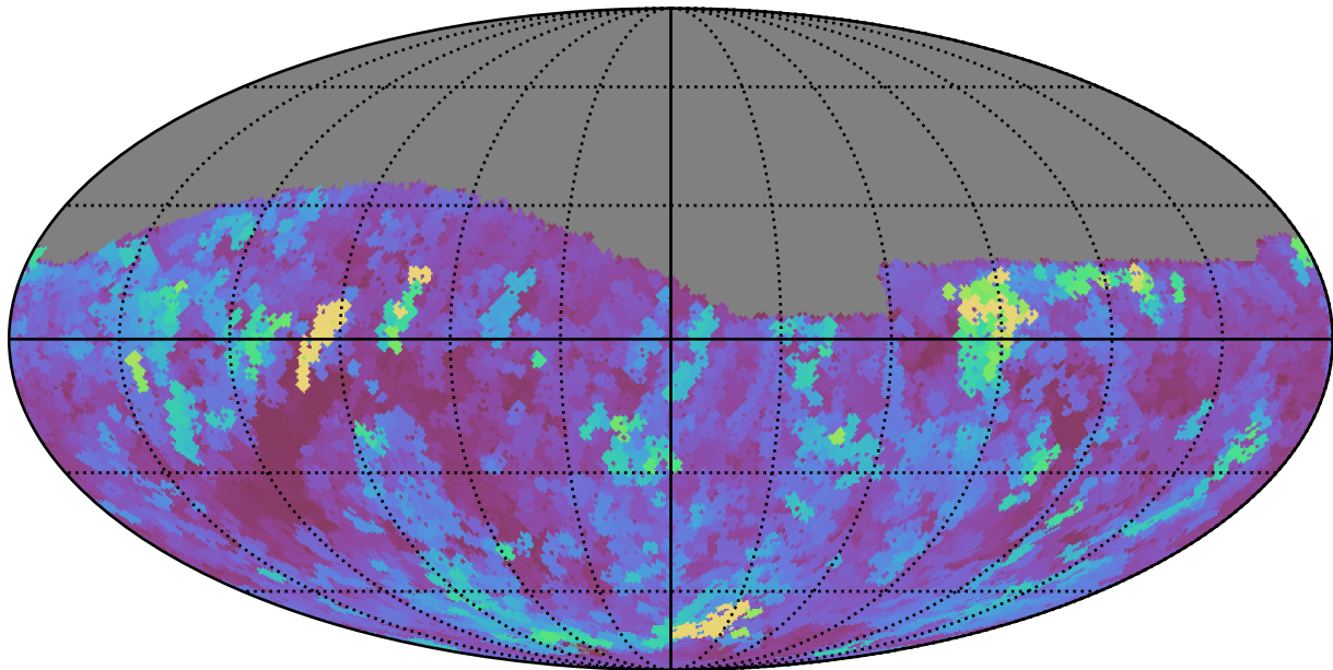
weather_cloudso20v3.4_10yrs Yr 1 r band: Max seeingEff
