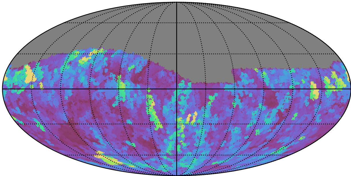
weather_cloudso20v3.4_10yrs Yr 1 i band: Max seeingEff
