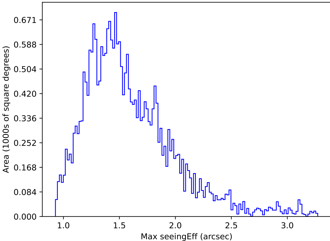
weather_cloudso20v3.4_10yrs Yr 1 i band: Max seeingEff
