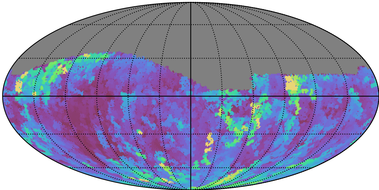
weather_cloudso20v3.4_10yrs Yr 1 g band: Max seeingEff
