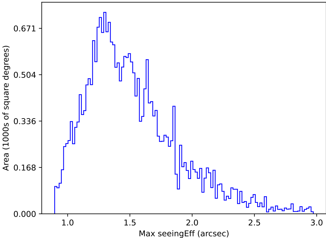
weather_cloudso20v3.4_10yrs Yr 1 g band: Max seeingEff
