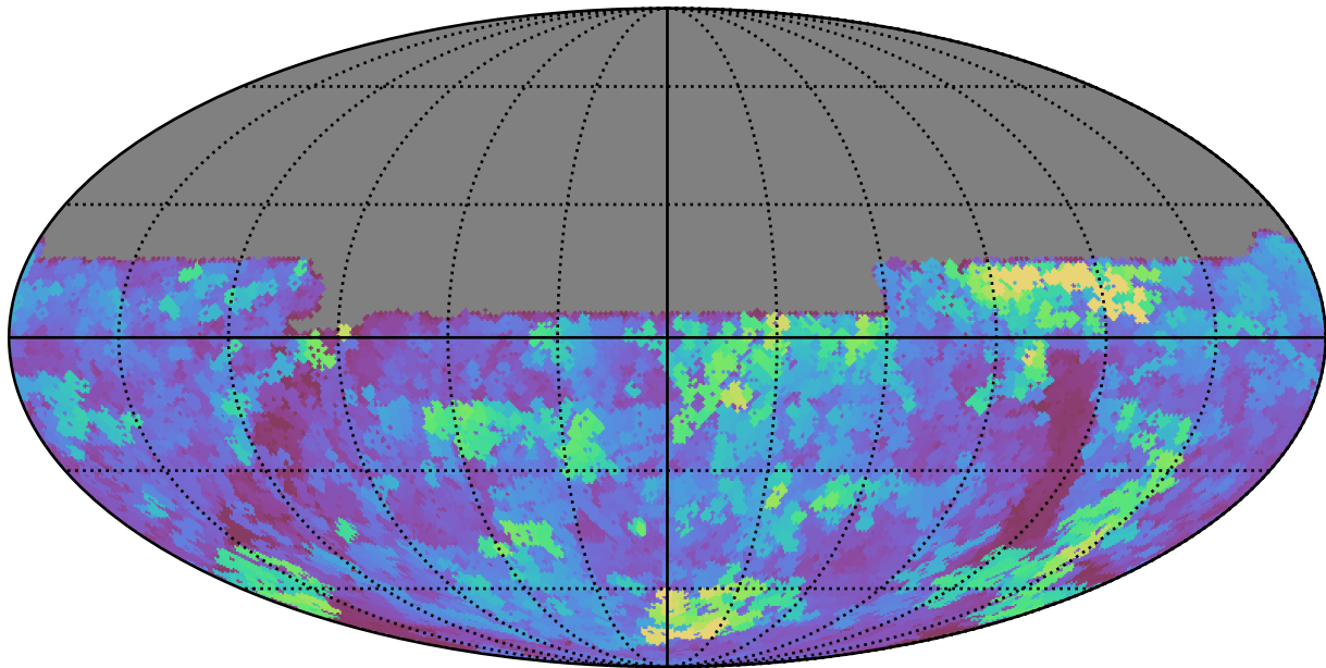
weather_cloudso20v3.4_10yrs All sky u band: Max seeingEff
