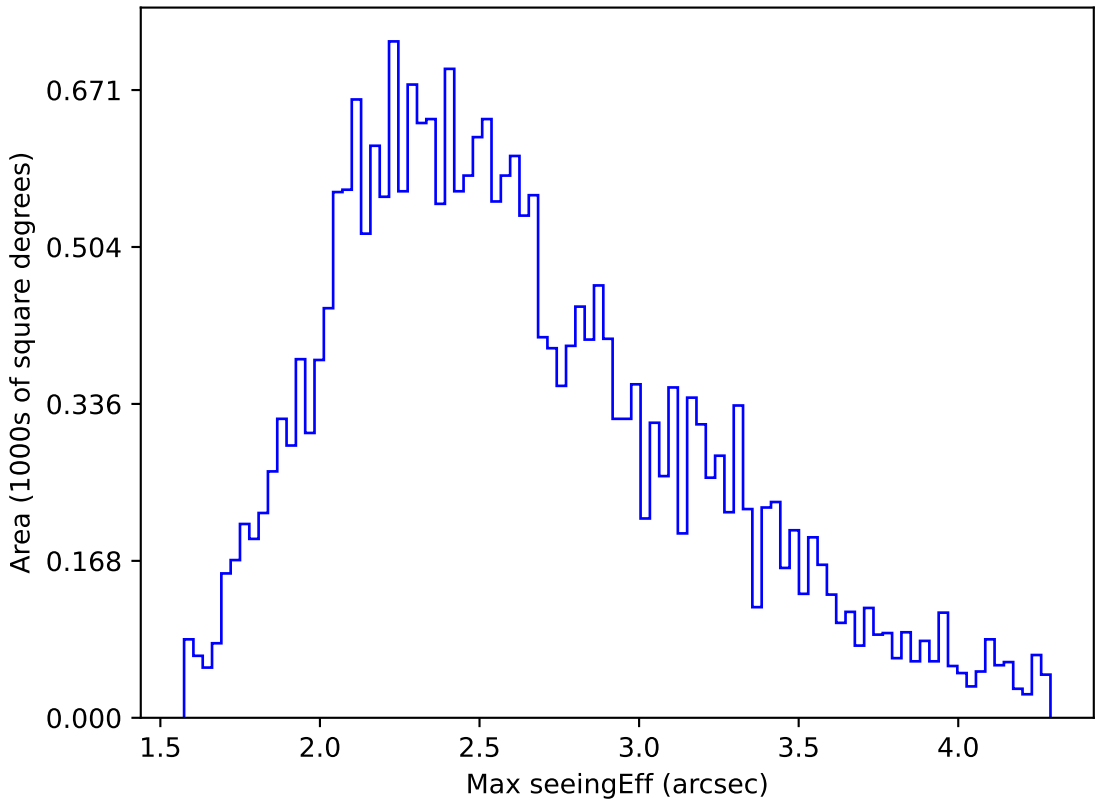
weather_cloudso20v3.4_10yrs All sky g band: Max seeingEff
