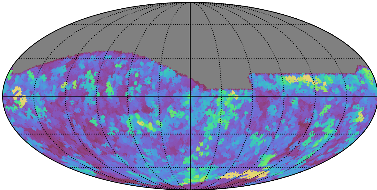
weather_cloudso20v3.4_10yrs All sky all bands: Max seeingEff
