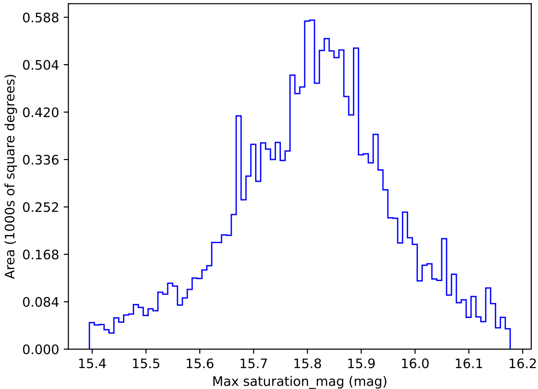
weather_cloudso20v3.4_10yrs WFD all bands: Max saturation_mag
