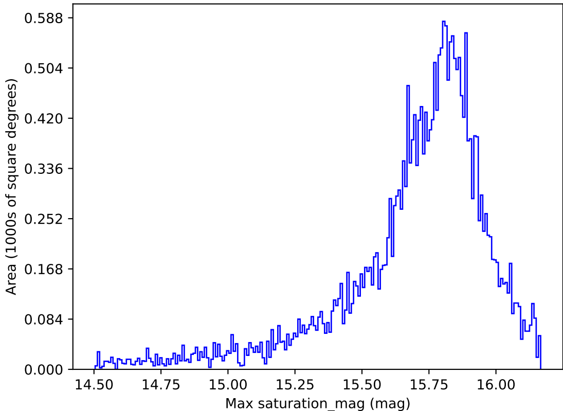
weather_cloudso20v3.4_10yrs All sky all bands: Max saturation_mag
