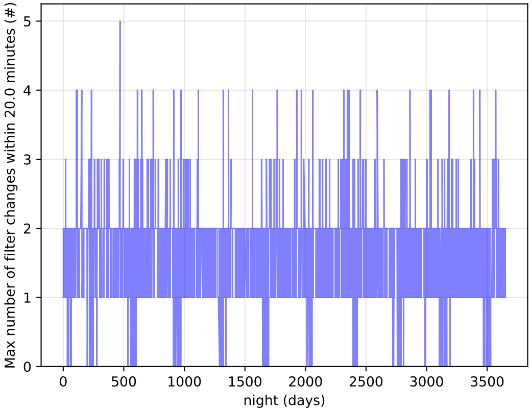
weather_cloudso20v3.4_10yrs Per Night: Max number of filter changes within 20.0 minutes
