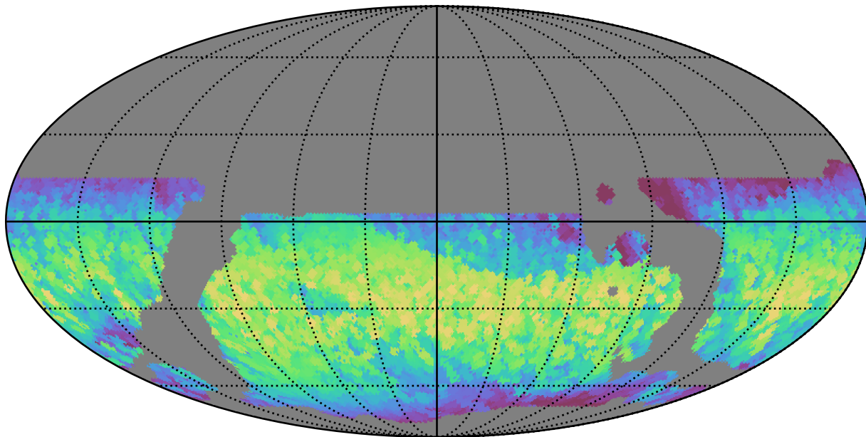
weather_cloudso20v3.4_10yrs WFD all bands: Max normairmass
