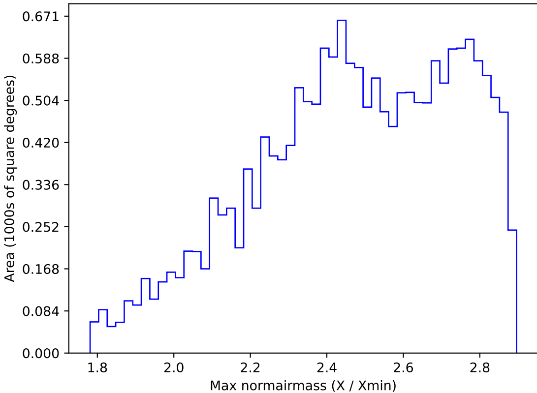
weather_cloudso20v3.4_10yrs WFD all bands: Max normairmass
