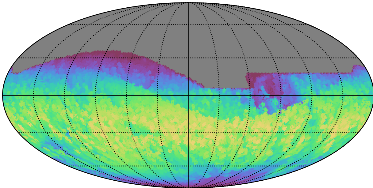
weather_cloudso20v3.4_10yrs All sky all bands: Max normairmass
