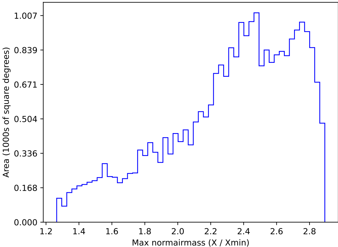
weather_cloudso20v3.4_10yrs All sky all bands: Max normairmass
