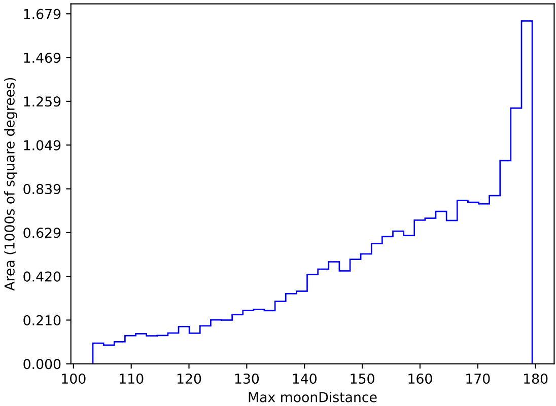
weather_cloudso20v3.4_10yrs WFD r band: Max moonDistance
