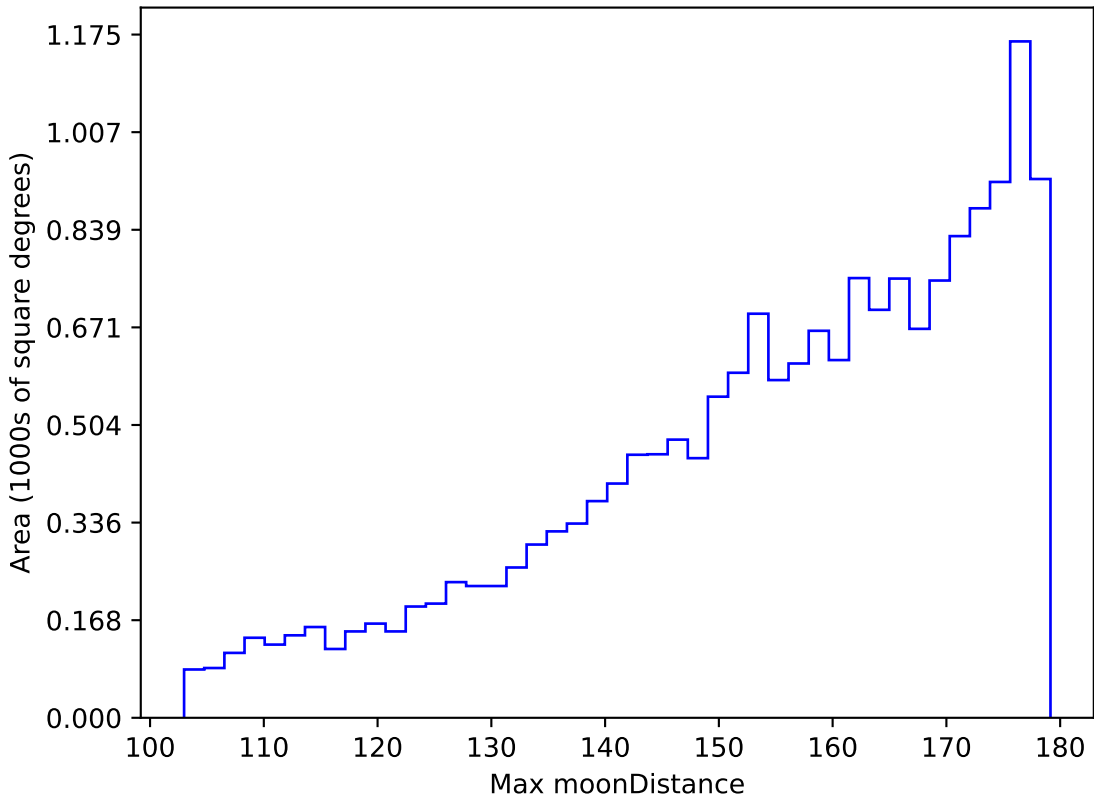
weather_cloudso20v3.4_10yrs WFD g band: Max moonDistance
