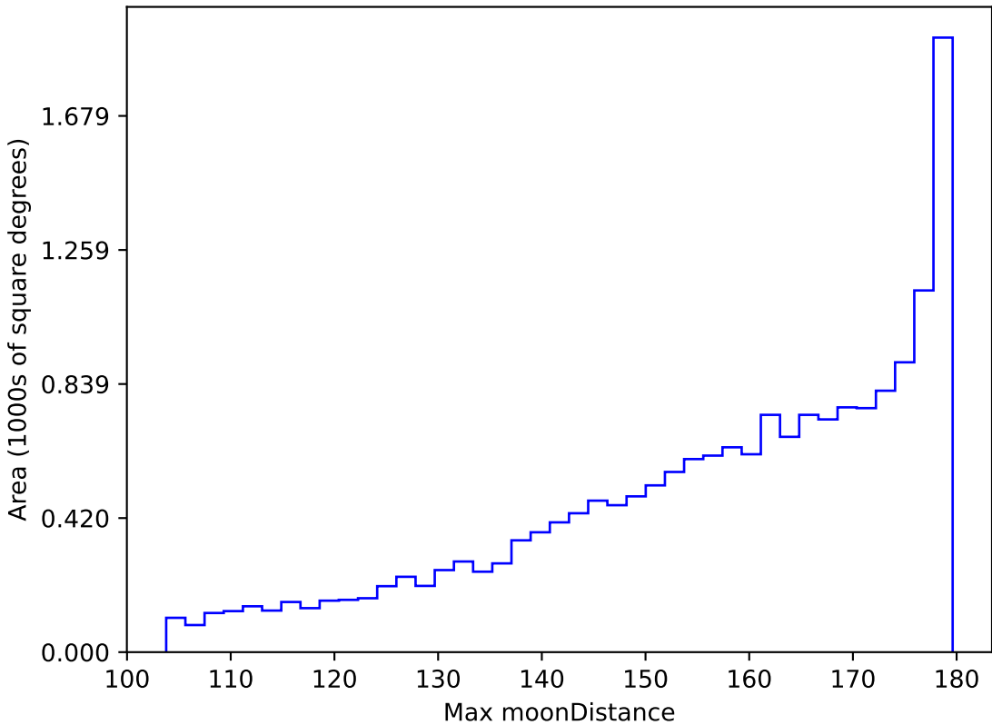
weather_cloudso20v3.4_10yrs WFD all bands: Max moonDistance
