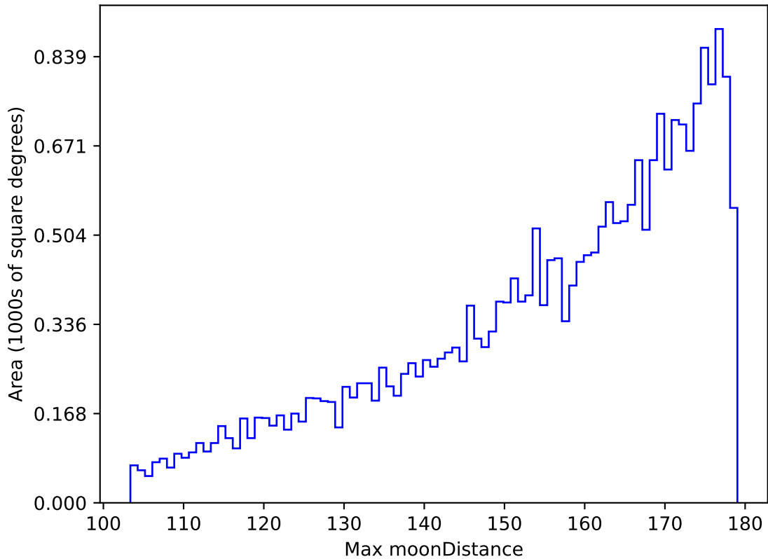
weather_cloudso20v3.4_10yrs All sky g band: Max moonDistance
