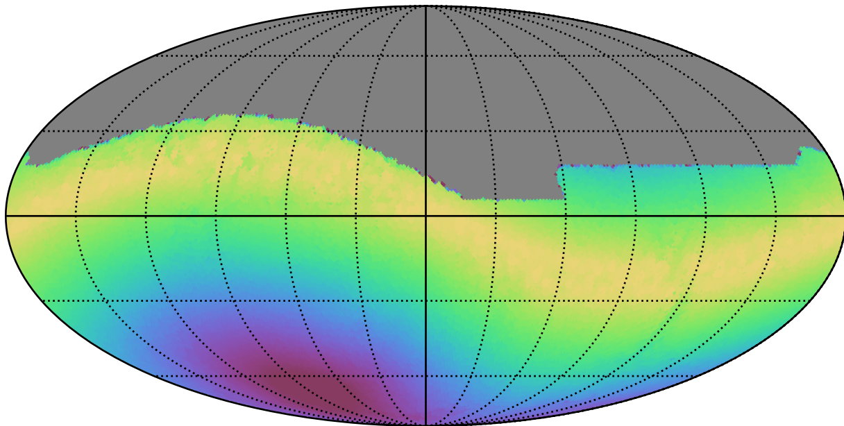
weather_cloudso20v3.4_10yrs All sky all bands: Max moonDistance
