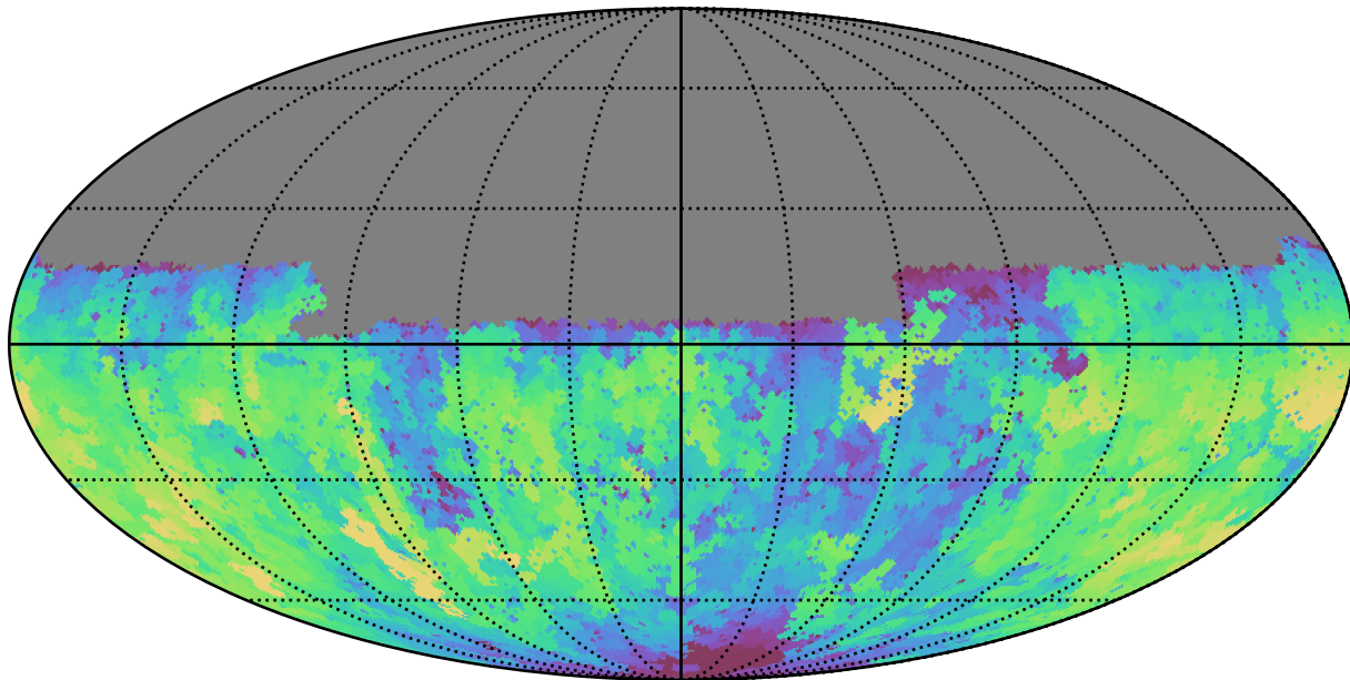
weather_cloudso20v3.4_10yrs Yr 1 u band: Max fiveSigmaDepth
