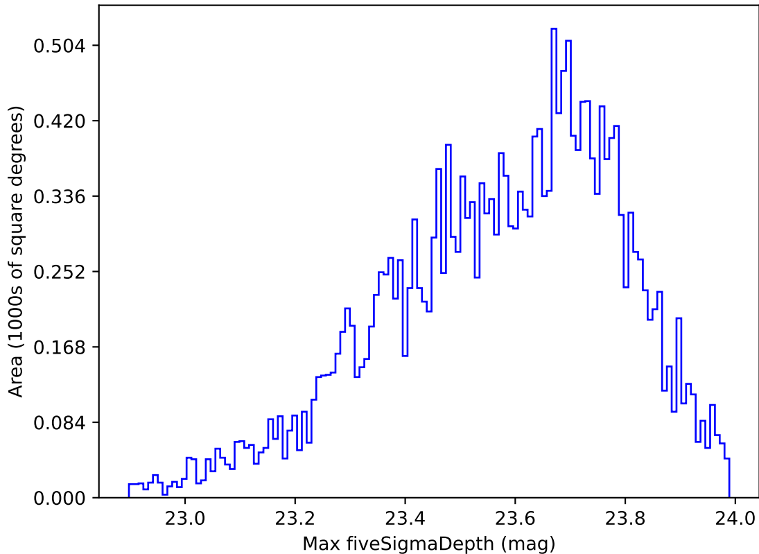
weather_cloudso20v3.4_10yrs Yr 1 u band: Max fiveSigmaDepth
