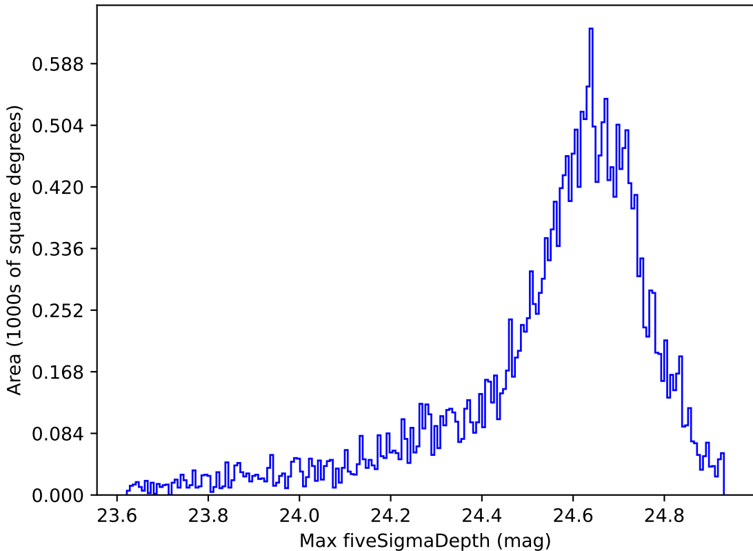
weather_cloudso20v3.4_10yrs Yr 1 r band: Max fiveSigmaDepth
