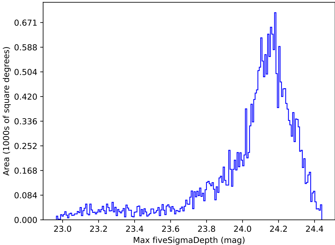
weather_cloudso20v3.4_10yrs Yr 1 i band: Max fiveSigmaDepth
