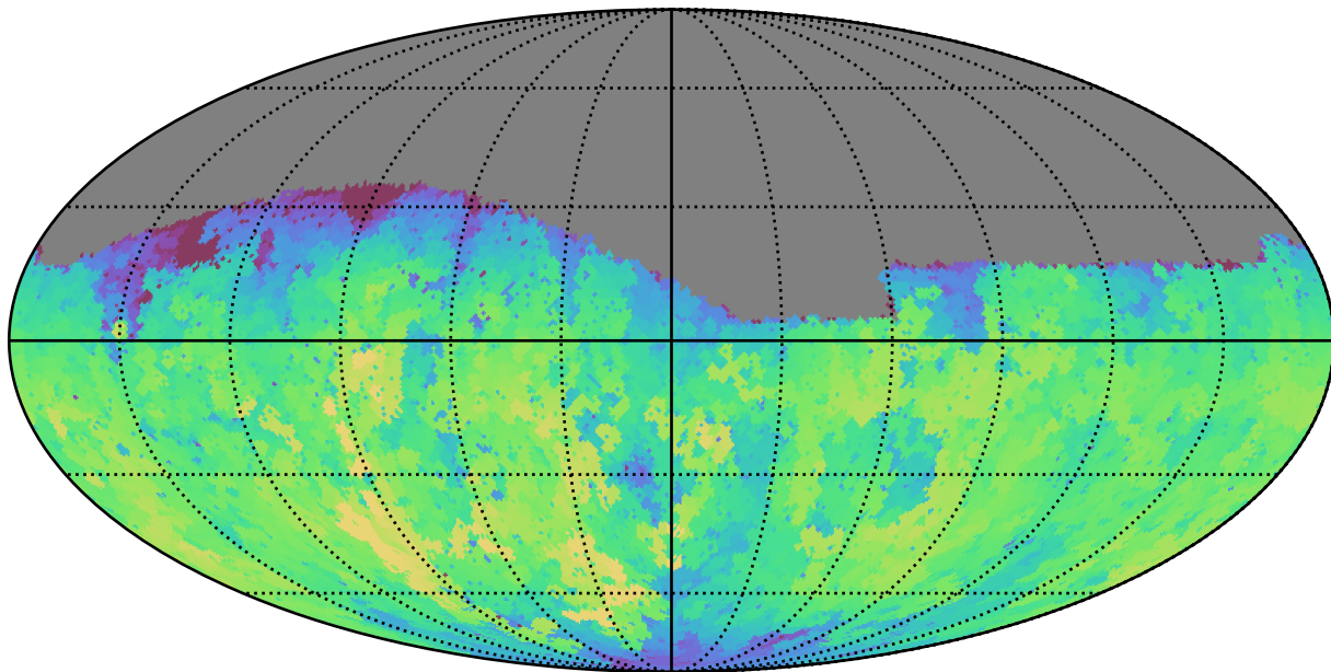
weather_cloudso20v3.4_10yrs Yr 1 g band: Max fiveSigmaDepth
