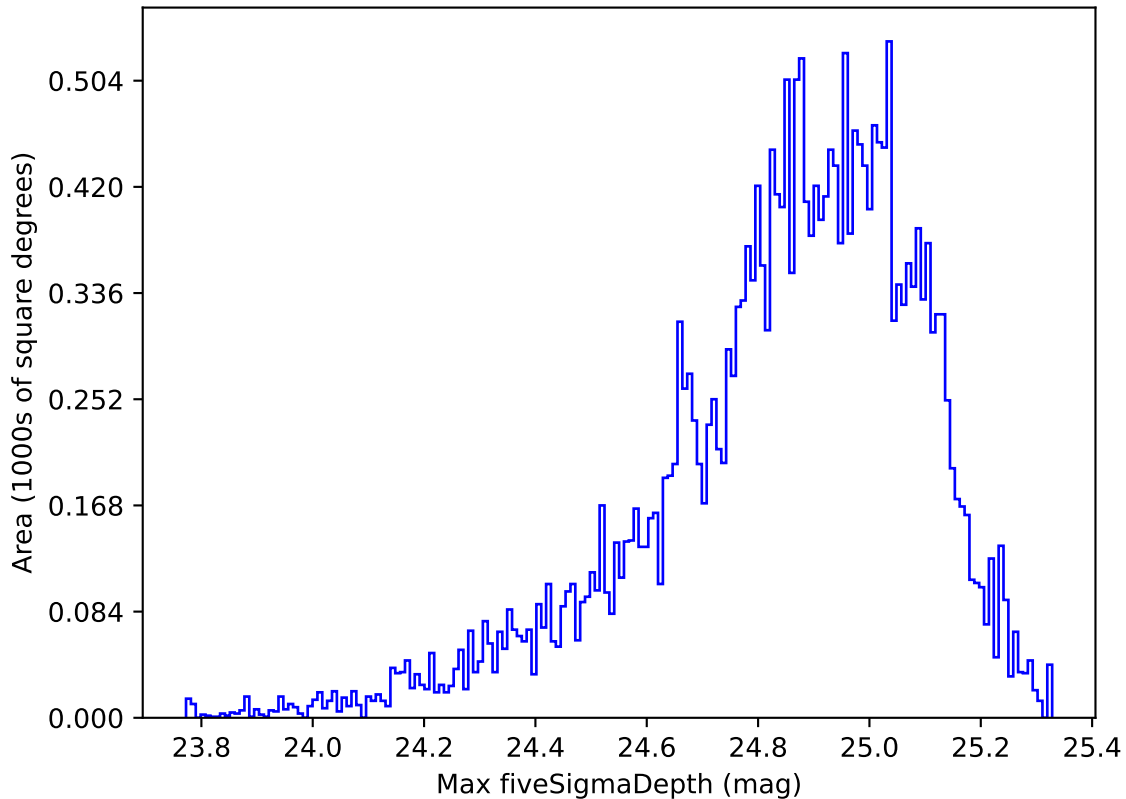
weather_cloudso20v3.4_10yrs Yr 1 g band: Max fiveSigmaDepth
