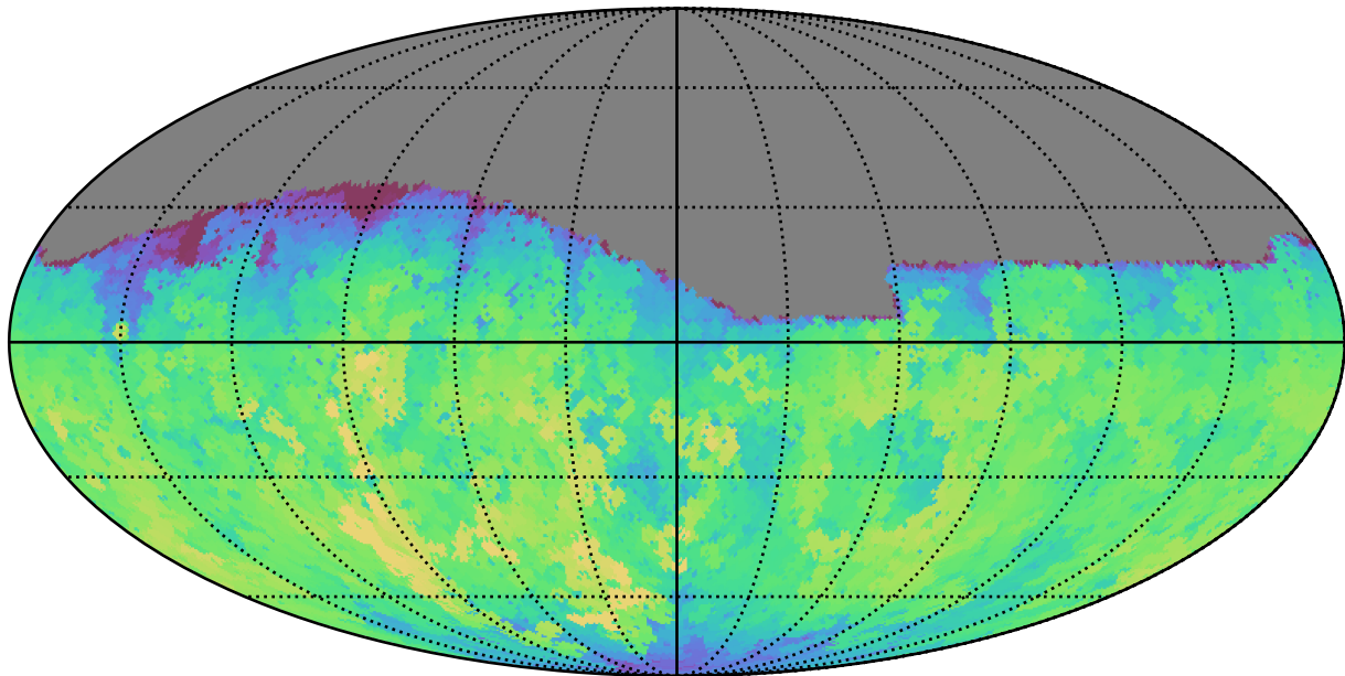
weather_cloudso20v3.4_10yrs Yr 1 all bands: Max fiveSigmaDepth
