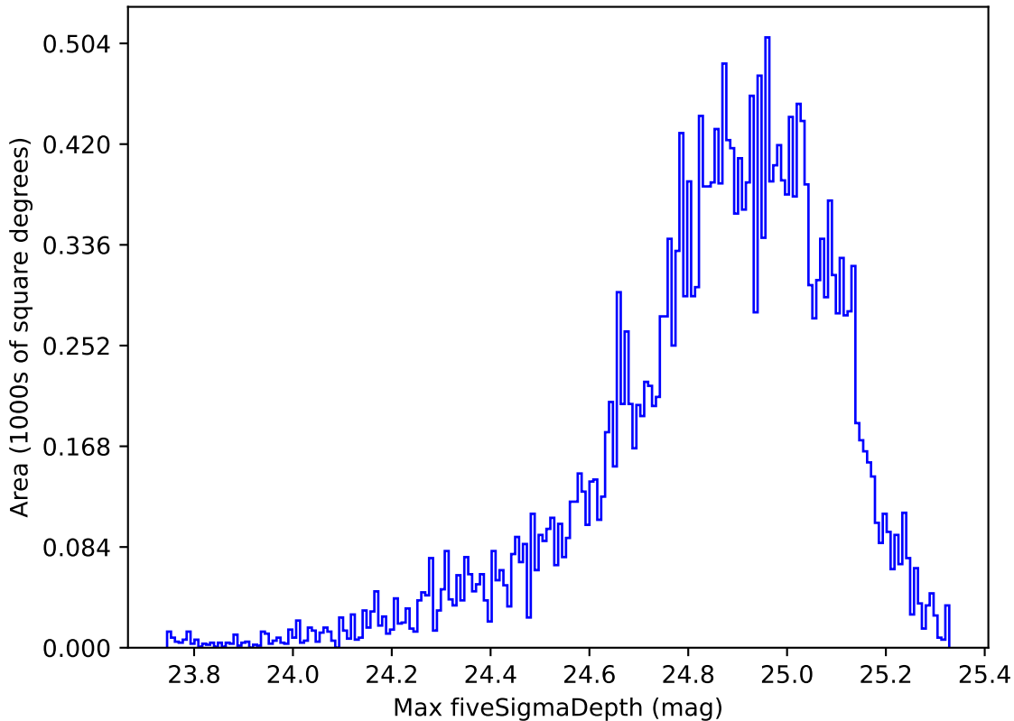
weather_cloudso20v3.4_10yrs Yr 1 all bands: Max fiveSigmaDepth
