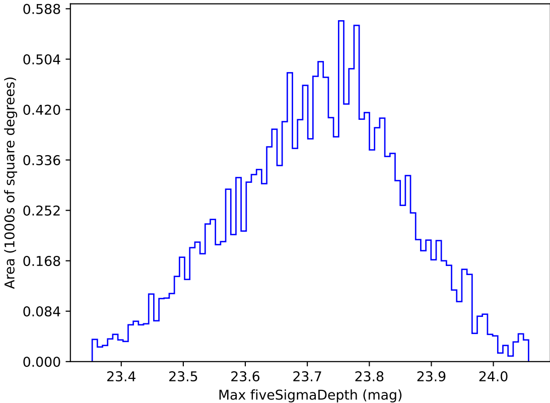
weather_cloudso20v3.4_10yrs WFD u band: Max fiveSigmaDepth
