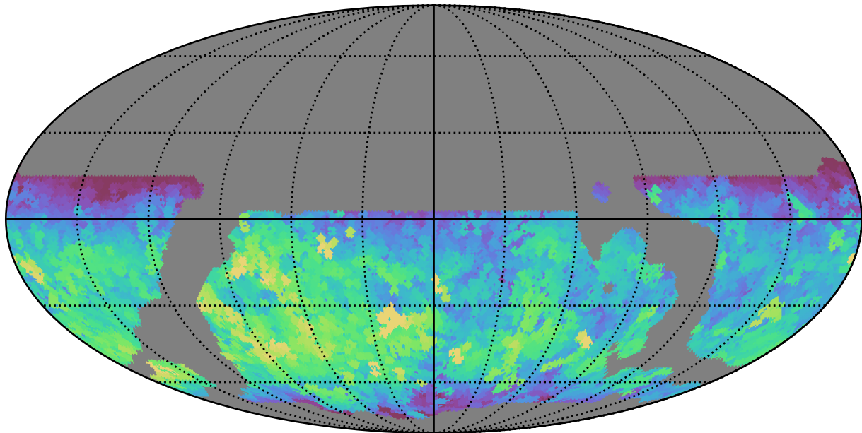
weather_cloudso20v3.4_10yrs WFD r band: Max fiveSigmaDepth
