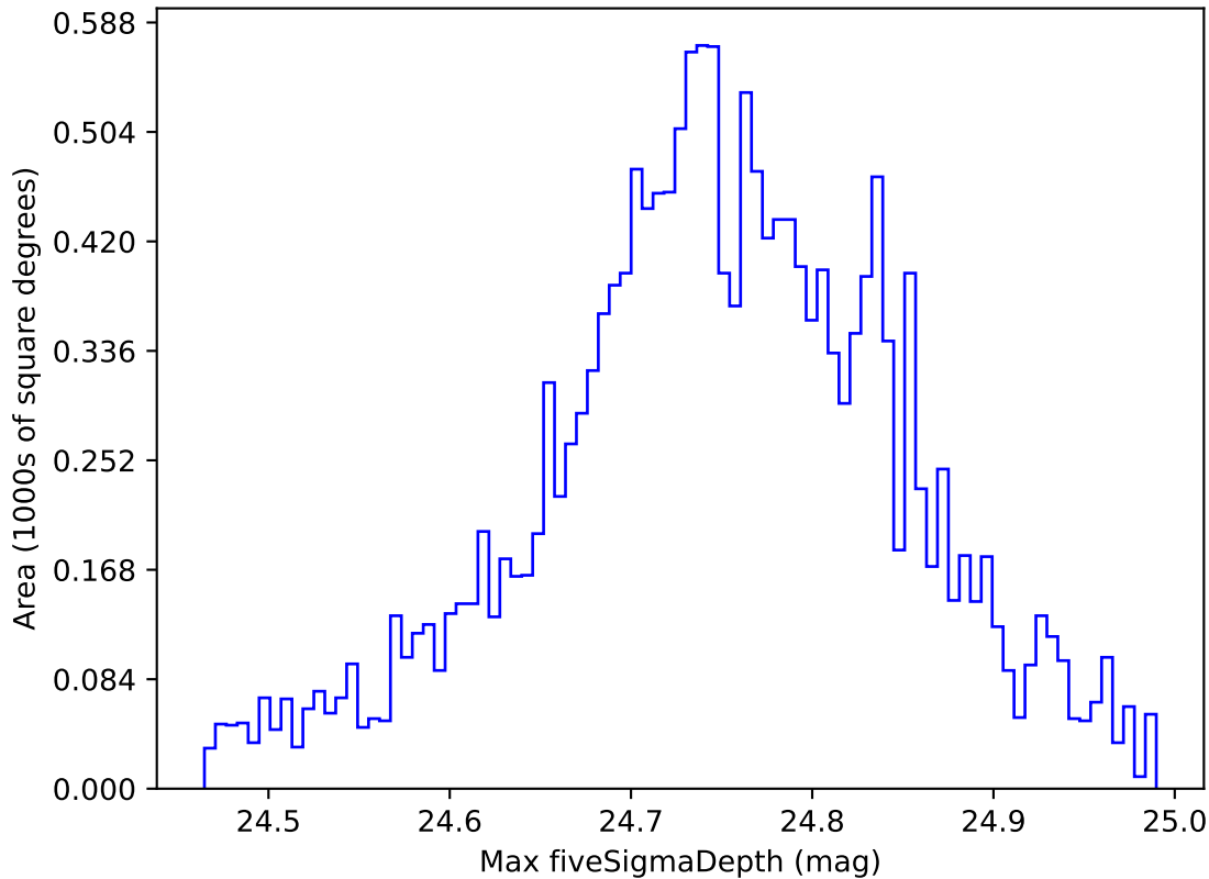
weather_cloudso20v3.4_10yrs WFD r band: Max fiveSigmaDepth
