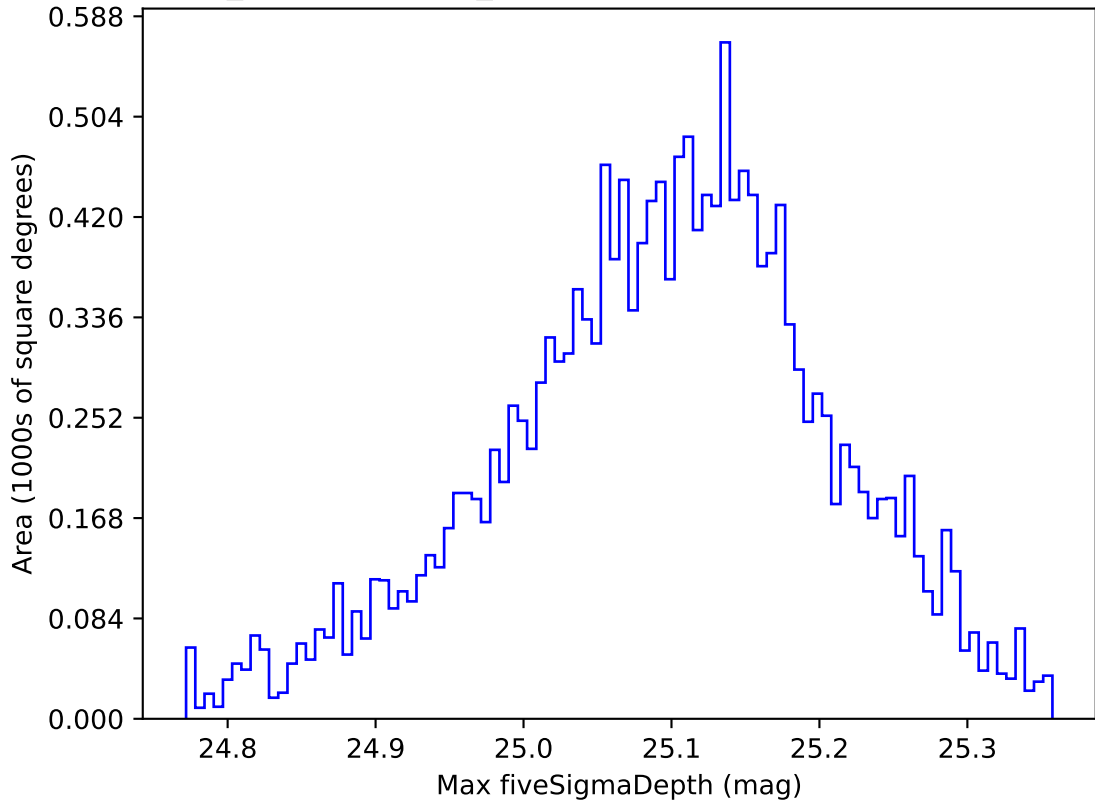
weather_cloudso20v3.4_10yrs WFD g band: Max fiveSigmaDepth
