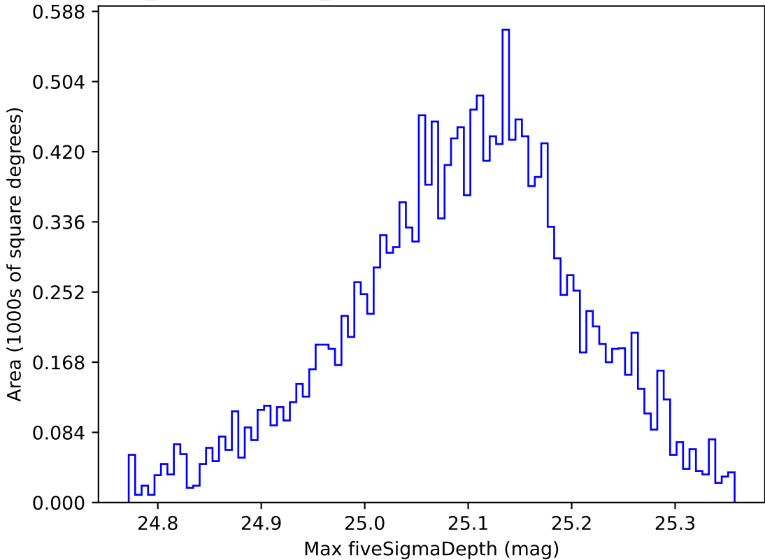
weather_cloudso20v3.4_10yrs WFD all bands: Max fiveSigmaDepth
