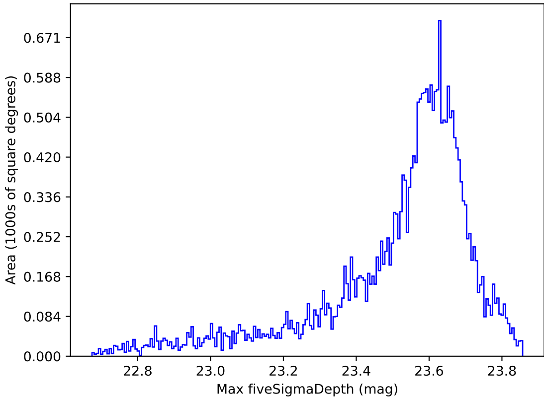
weather_cloudso20v3.4_10yrs All sky z band: Max fiveSigmaDepth
